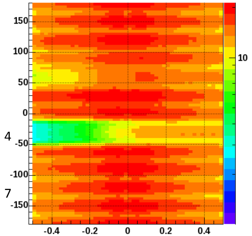
\phi versus \eta for Sti
