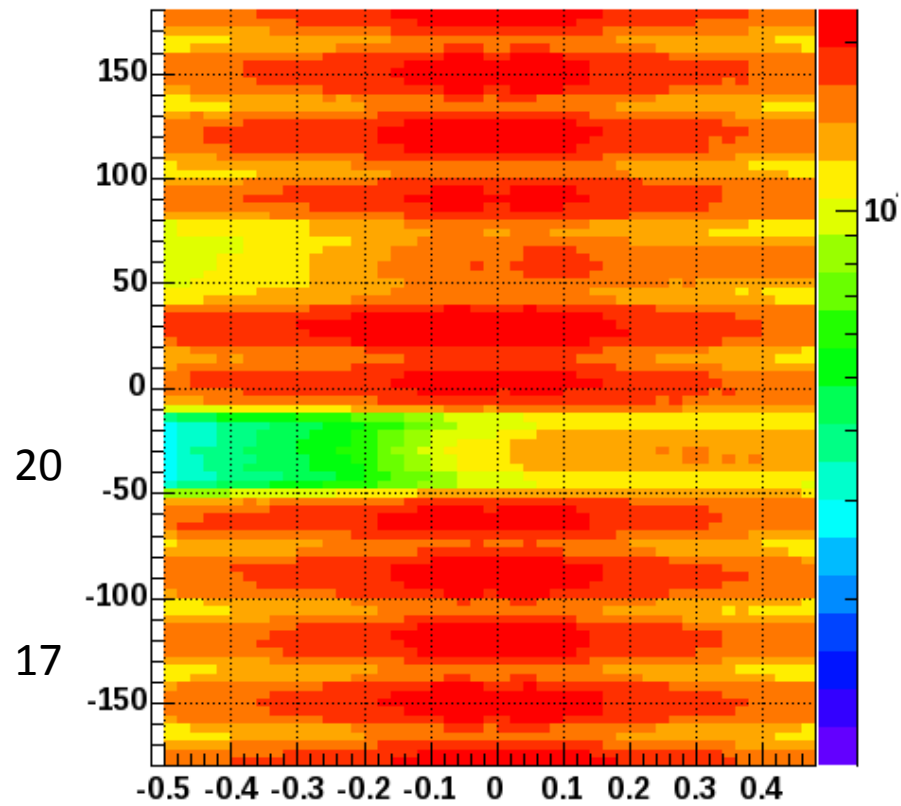
\phi versus \eta for StiCA
